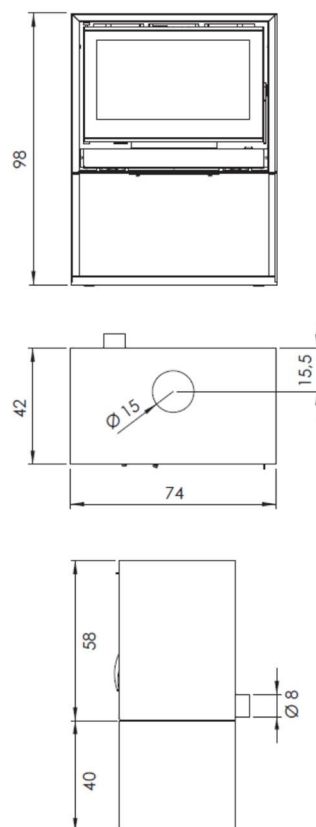
RK-70 LEÑERA RK-70 WITH LOG STORE
