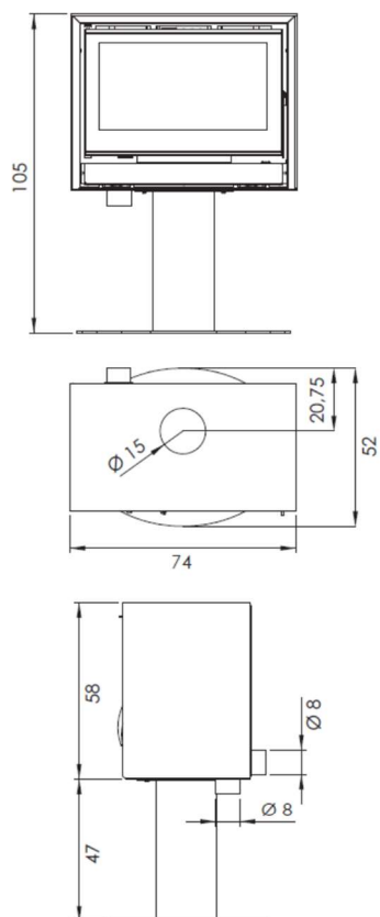
RK-70 PIE RK-70 FREE-STANDING
