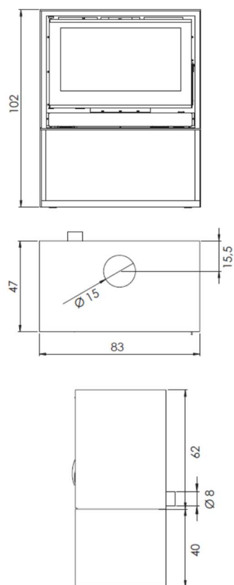
RK-80 LEÑERA RK-80 WITH LOG STORE
