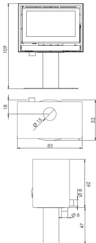
RK-80 PIE RK-80 FREE-STANDING
